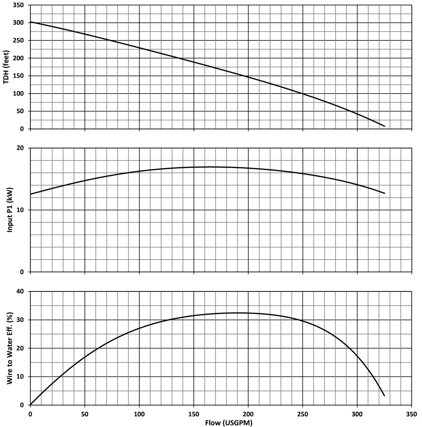
Pump Performance Test - US Units
