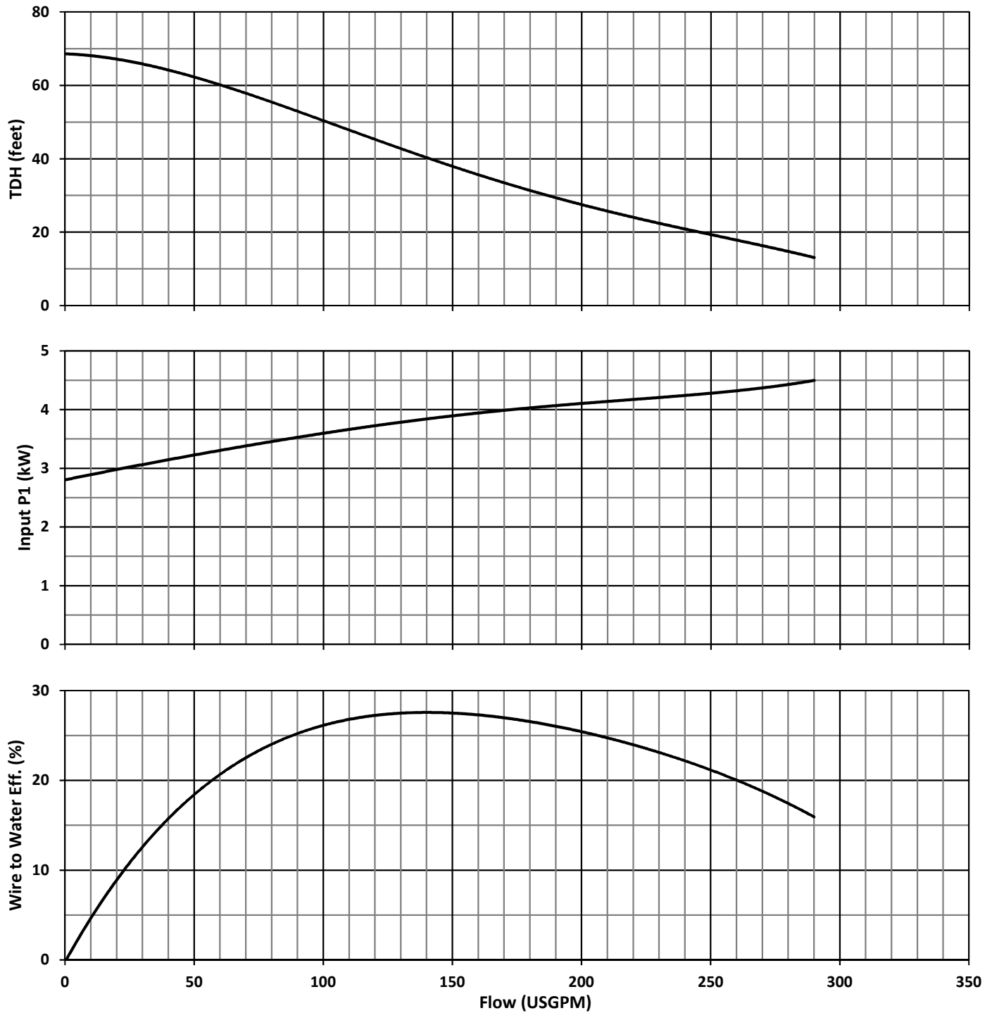
Pump Performance Test - US Units
